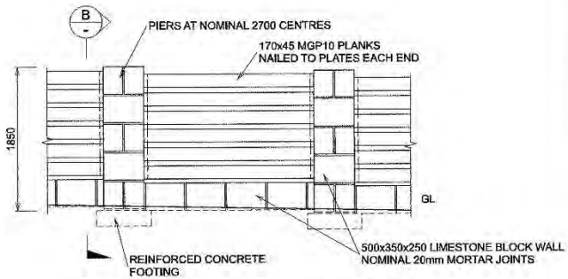
TYPICAL WALL ELEVATION
