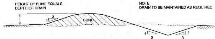
CUTOFF DRAIN
