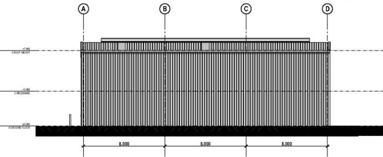
4 WEST ELEVATION Scale 1:100
